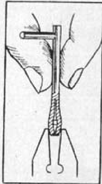
FIG. 58. TIGHTENING THE NEEDLE ROD
