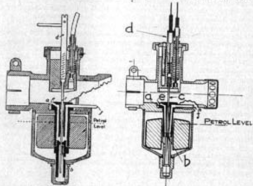
FIGS. 51 AND 52. SHOWING LEFT AND RIGHT, RESPECTIVELY, SECTIONAL VIEWS OF SINGLE AND DOUBLE LEVER CARBURATORS
