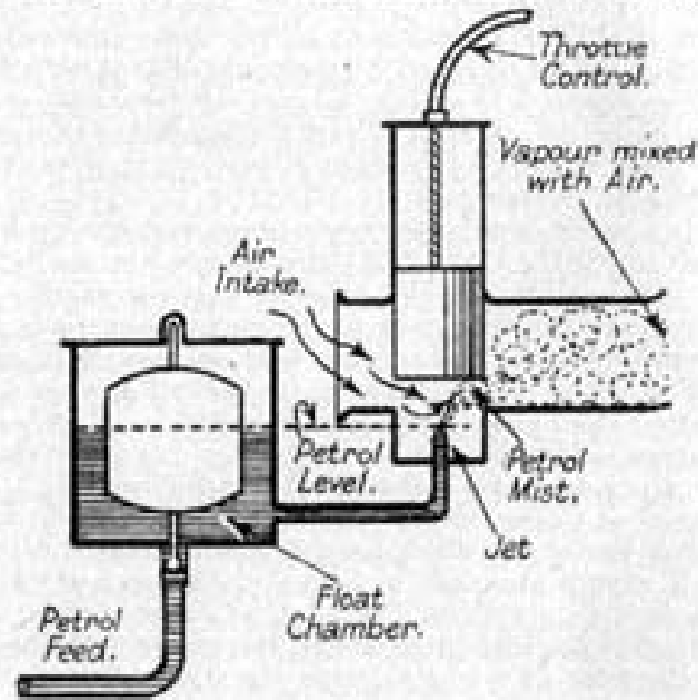
FIG. 50. DIAGRAM EXPLAINING THE PRINCIPLE OF CARBURATION
