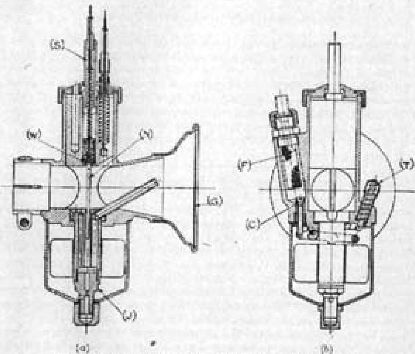
FIG. 60A. THE VILLIERS HEAVYWEIGHT CARBURETTOR.
