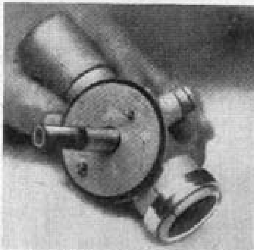
FIG. 55. FUEL NEEDLE IN POSITION (KARLISCH TYPE)
