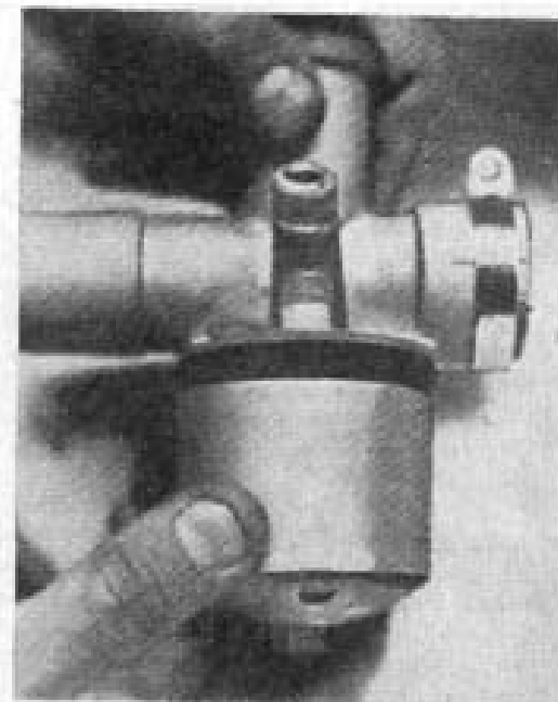
FIG. 56. WHEN DISMANTLING THE VILLIERS CARBURETTOR, BE CAREFUL THAT THE FUEL NEEDLE IS NOT LOST
